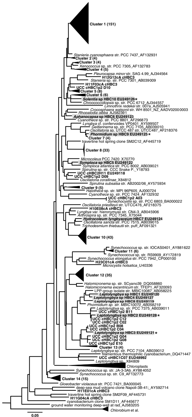
Figure 6 Phylogenetic tree of cyanobacterial 16S ribosomal RNA gene sequences recovered from clone libraries generated with different primer sets and from isolates, as described in the text. Short clone sequences and longer isolate sequences were inserted into a large tree based on full or nearly full 16S rRNA gene sequences using parsimony and filtering the data with a 50% cyanobacterial conservation filter while maintaining the overall tree topology. Clusters containing at least four environmental sequences recovered in this study were compressed. The number of sequences included in each cluster is enclosed in parentheses. The scale bar represents 0.05 substitutions per nucleotide position. Highborne Cay cultivars are highlighted in gray and cultivars detected in the cultivation-independent clone libraries are indicated with asterisk.
